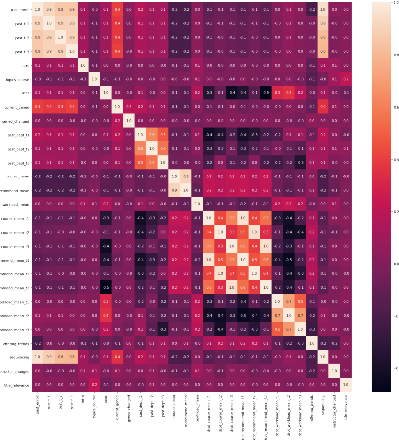
Figure 3.2: A visualization of the feature correlation matrix. Flag values were excluded for readability and relevancy. Data are labeled with their Pearson correlation coefficient.
